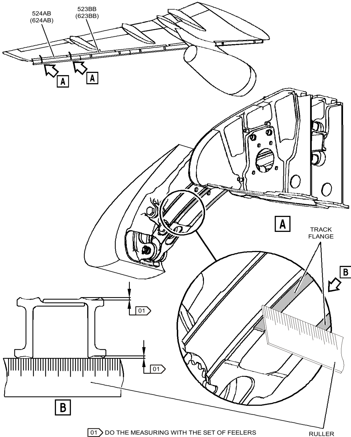
Measuring of the track wear Figure 602
