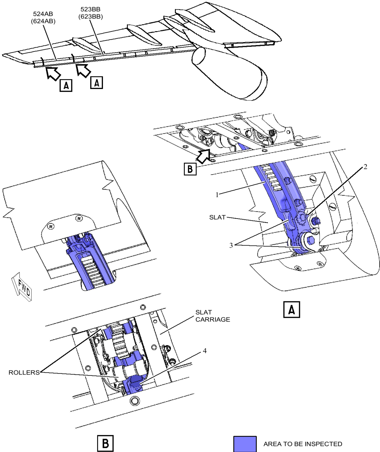
Detailed Inspection of the Slat Section 4 Tracks 8 and 9 Figure 601
